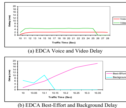
Figure 5. Network performance using default EDCA parameters.
